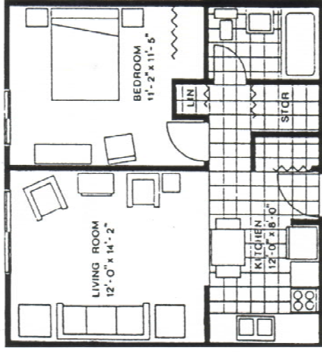
A typical floor plan
